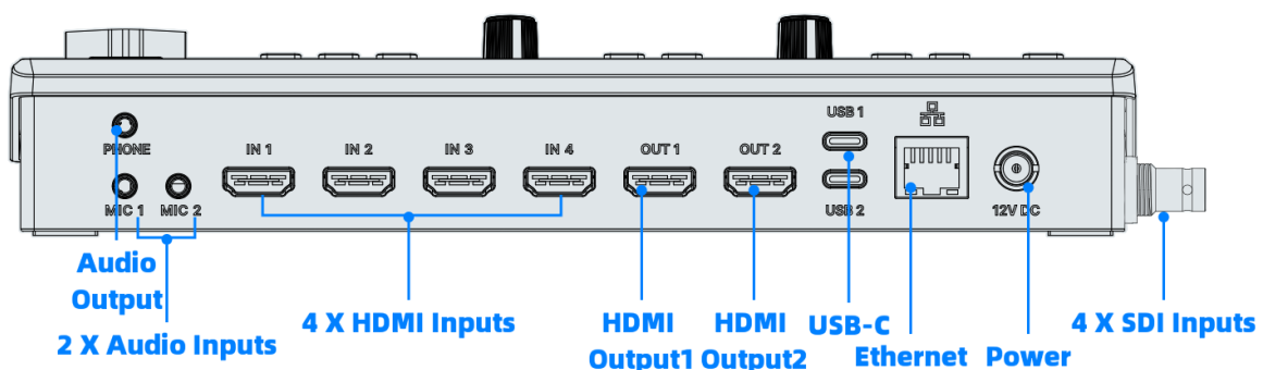
Figure 4.2-1 Connectors on the Rear
