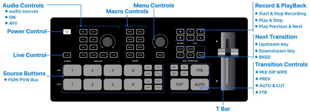
Figure 4.1-1 GoStream Panel
