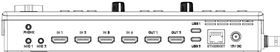
Figure 6-6 Rear Panel(Unit: mm)
