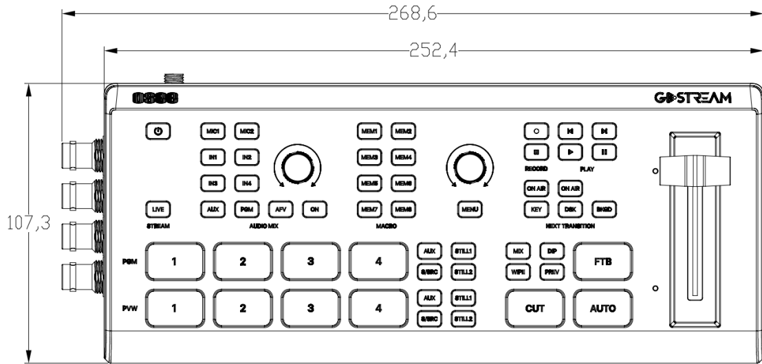
Figure 6-5 Front Panel(Unit: mm)
