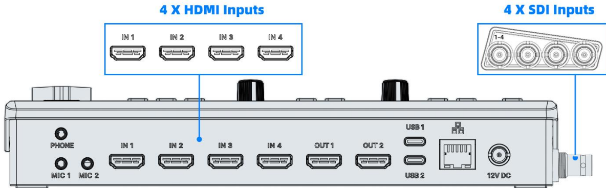
Figure 4.2-3 HDMI Inputs
