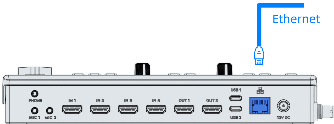
Figure 4.1-74 Ethernet Connection
