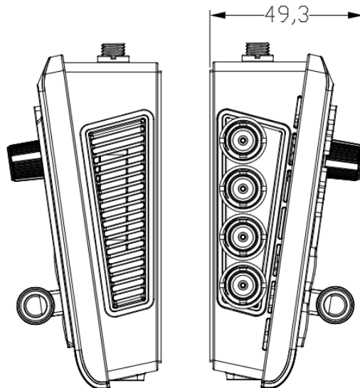
Figure 6-7 Side View(Unit: mm)
